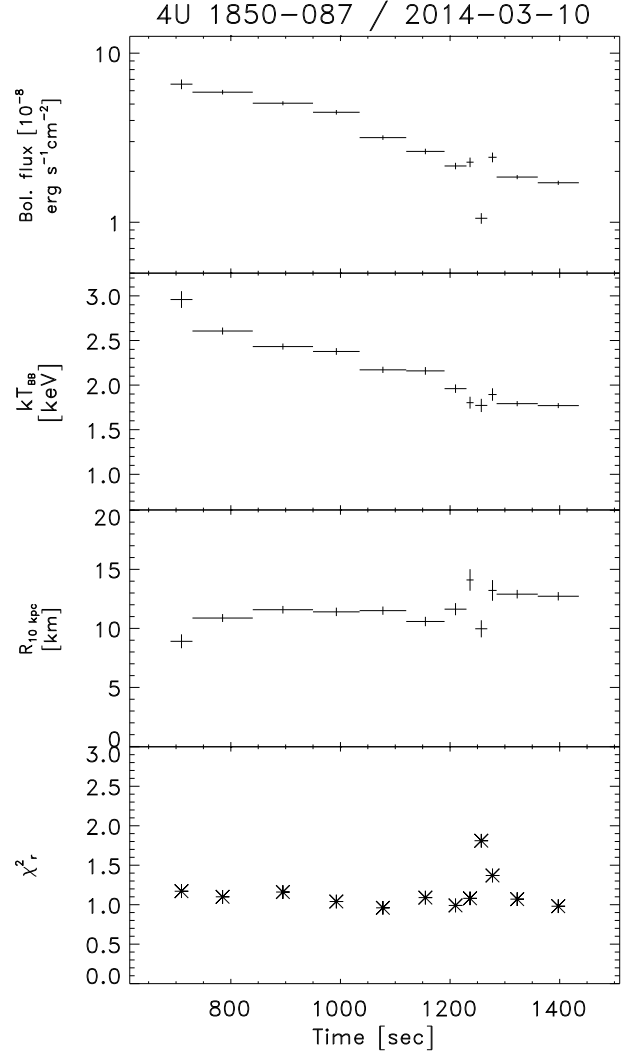
Fig. 10: 4U 1850-087: Time-resolved spectroscopy.
