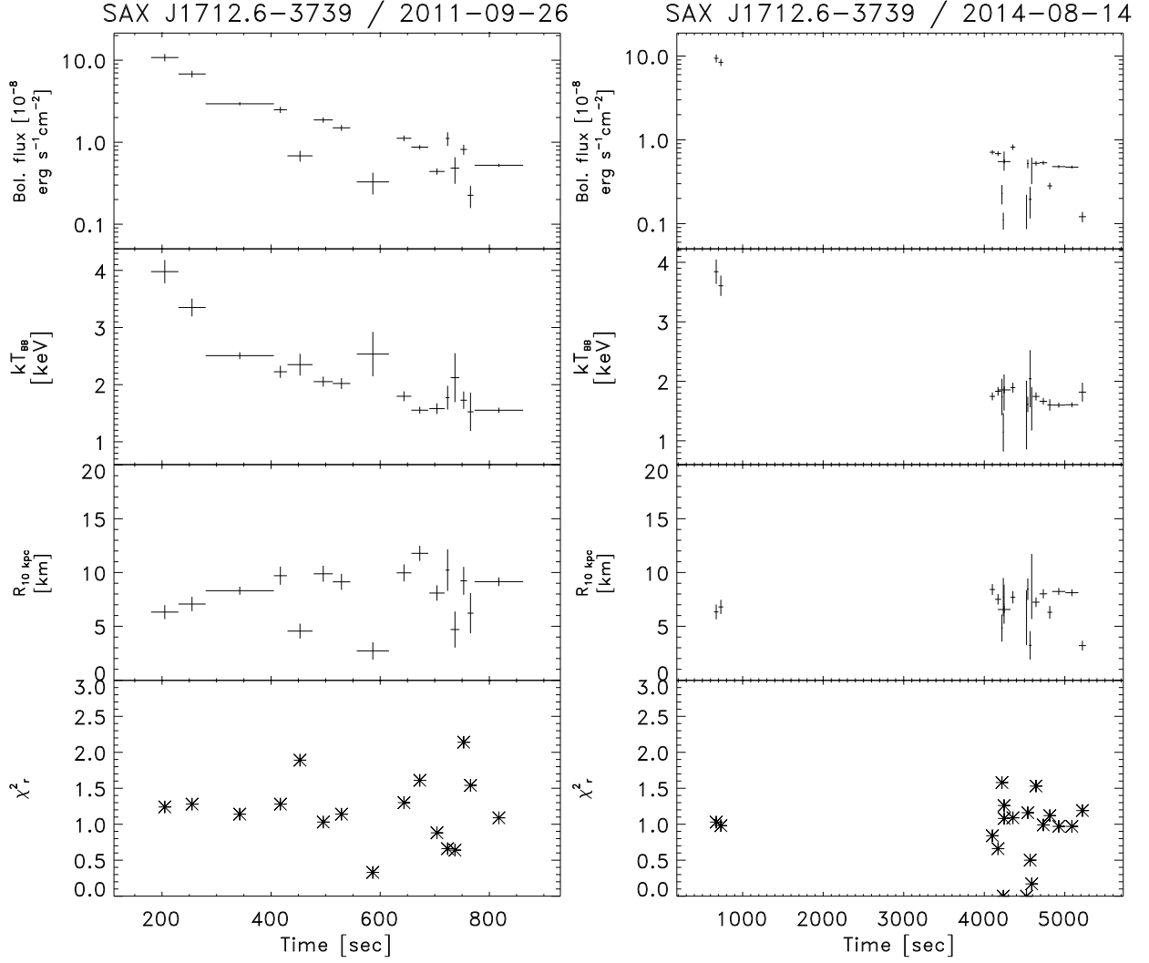
Fig. 6: SAX J1712.6-3739: Time-resolved spectroscopy of both long bursts.
