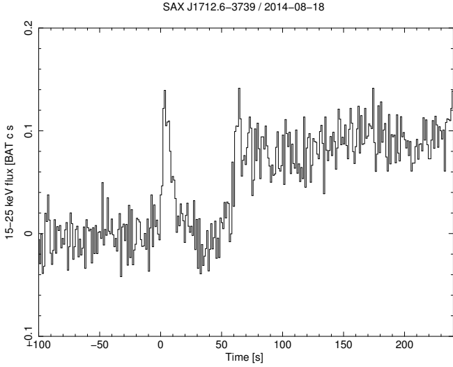
Fig. 7: BAT light curve of the third burst from SAX J1712.6-3739, reconstructed from rate meter data in 15–25 keV (pre-burst flux subtracted between -40 and 0 s from burst start and normalized to projected detector area as seen from source). During this data stretch BAT had a fixed pointing.
