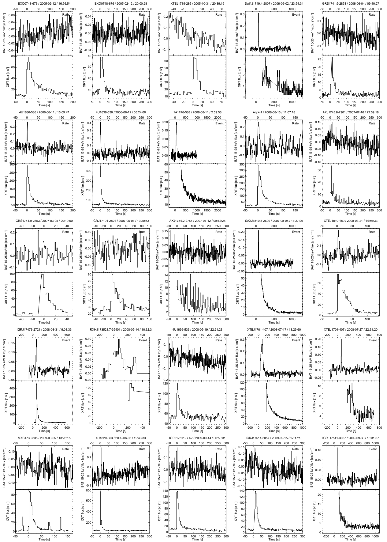
Fig. A.1: BAT (upper panels) and XRT light curves (lower panels) of all 90 X-ray bursts that have XRT coverage. The BAT light curves are labeled 'Event' if they are from mask-tagged event data or 'Rate' if they are inferred from rate meter data. In the latter case, the rate meter data have been pre-burst subtracted and divided by the photon-collecting area illuminated by the source that was identified on board.
