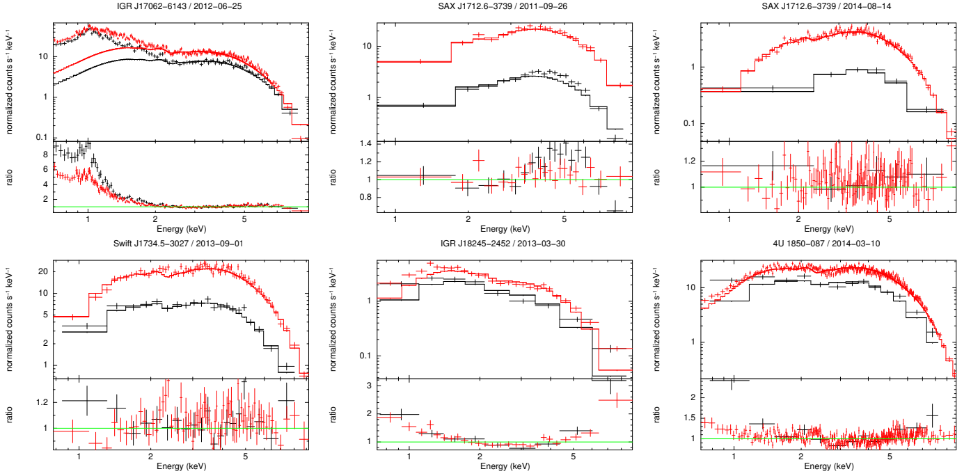
Fig. 3: Spectra of the upward and downward fluctuations for the six selected bursts. For IGR J17062-6143, only data above 2 keV were fitted. The lower panels show the ratio of the data to the applied model. Black data points are for ‘lo’ data, red for the ‘hi’.
