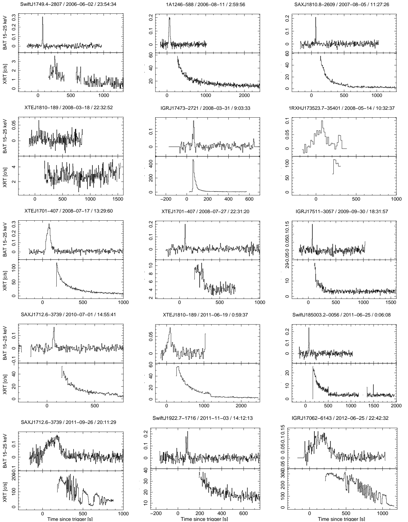
Fig. 1: BAT and XRT light curves of all 28 X-ray bursts with BAT event files and followed up with XRT, except 4U 1812-12/2005-02-24 because its XRT coverage is sparse. The BAT light curves are normalized and corrected for a changing pointing due to the slews. The XRT data are for the complete detector and without corrections for pile-up or background. The steps that can sometimes be seen in XRT data are due to a switch in CCD data collection mode with different pile-up fractions.
