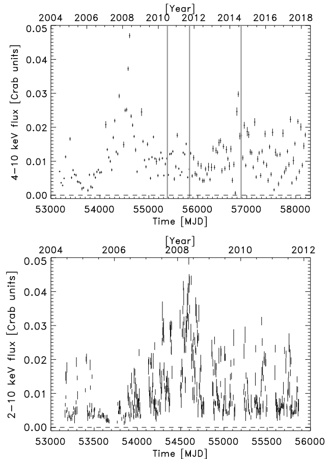
Fig. 5: (Top) 4–10 keV light curve over 14 years for SAX J1712.6-3739 with a time resolution of 1 month. The data are from the PCA Bulge Scan program (Swank & Markwardt 2001) between 2004 and 2012, and MAXI observations between 2009 and 2018 (e.g., Negoro et al. 2016). A cross calibration has been performed for the two years that the programs overlap. Strong variability is obvious. Vertical bars indicate the times of the three bursts detected with Swift. (Bottom) 2–10 keV light curve measurements with PCA over 8 years for SAX J1712.6-3739. Typically, each data point represents 1 min of data and measurements were performed twice a week. Strong variability is also obvious at this resolution.
