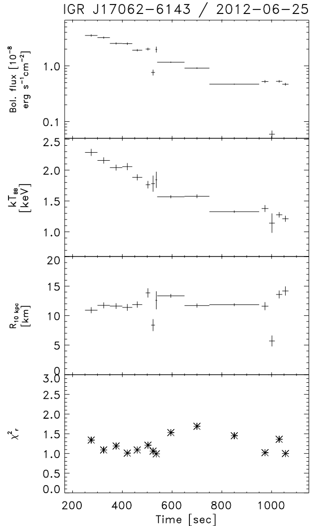
Fig. 4: IGR J17062-6143: Time-resolved spectroscopy
