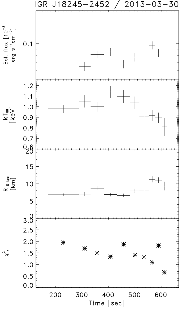
Fig. 9: IGR J18245-2452: Time-resolved spectroscopy.
