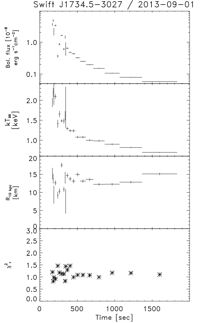
Fig. 8: Swift J1734.5-3027: Time-resolved spectroscopy.
