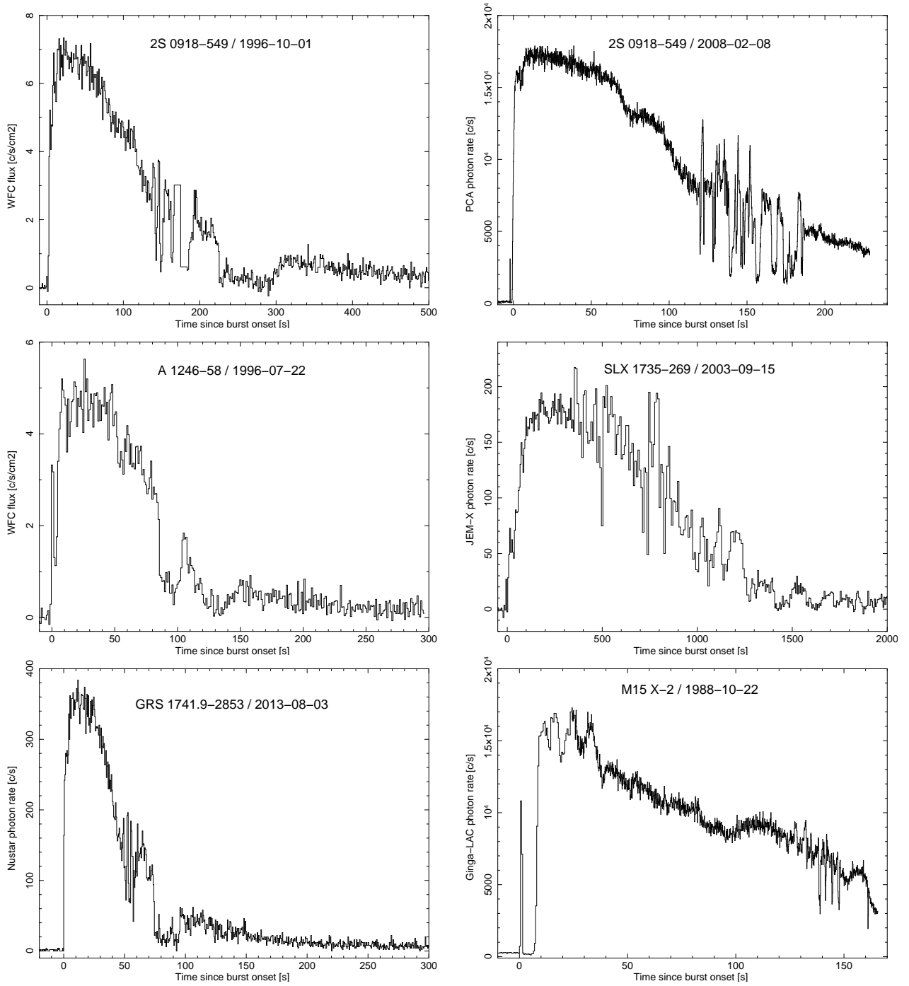
Fig. 11: Light curves of literature bursts with fluctuations.
